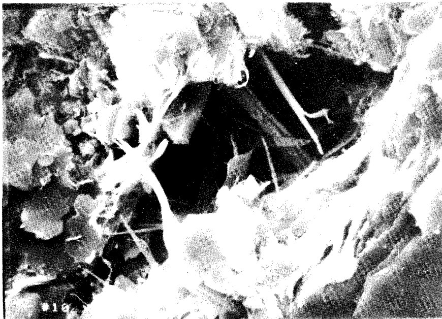
Figure 6. Photomicrograph of convection oven dried core sample from 3,530 feet, showing well developed fibrous illites (2,400 X). Long dimension of photo is 50 microns.
